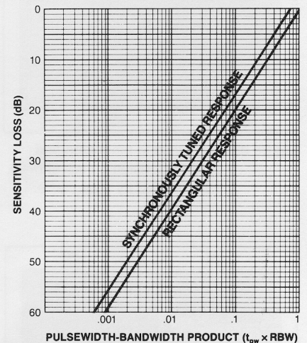
Figure 29. Sensitivity loss of pulsed signals vs CW.
