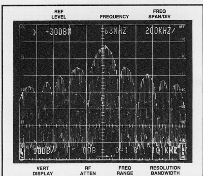
Figure 31. FM'ing carrier.
