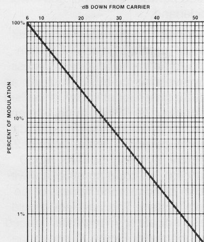
Figure 13. Chart of dB vs. % of Modulation.
