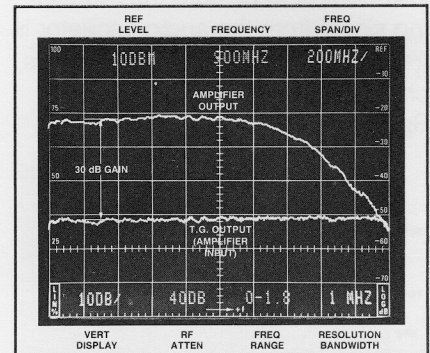
Figure 24. Amplifier response to SA/TG system.
