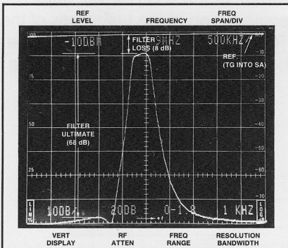
Figure 21. Filter response of filter using SA/TG.
