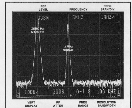
Spectrum Analyzer Waveform: 3 MHz Sine Wave
