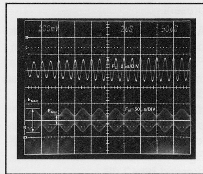
Figure 11. AM Modulation (50%) in time domain.
