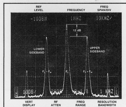
Figure 12. AM Modulation in frequency domain.
