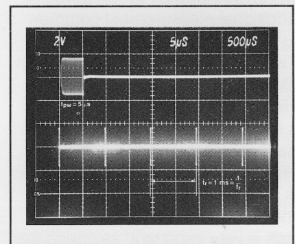
Figure 25. Time domain display of pulse waveform.
