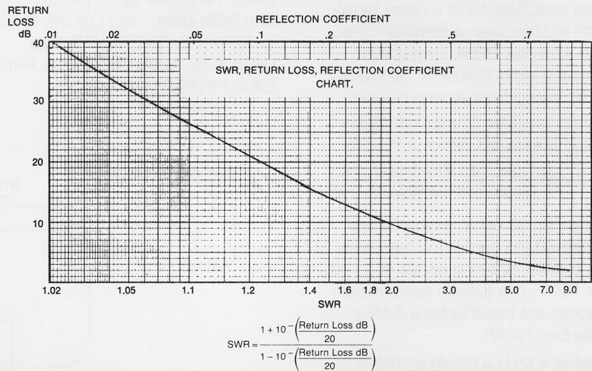
Figure 36. SWR, Return Loss, and Reflection Coefficient Chart.
