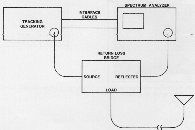
Figure 34. SWR test setup.
